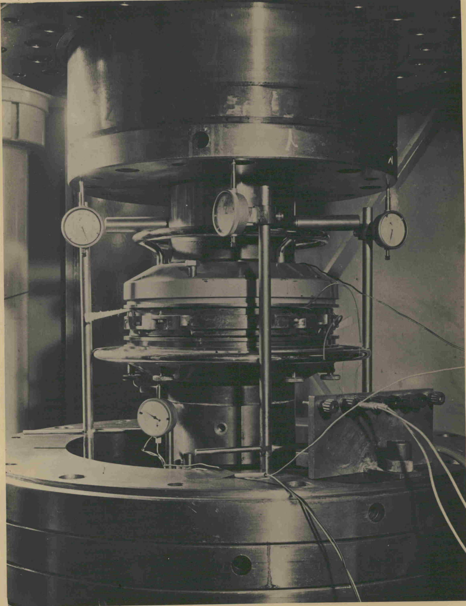
Fig.3 Photograph of the "X type anvil" showing the four dial gages used to record the piston displacements
