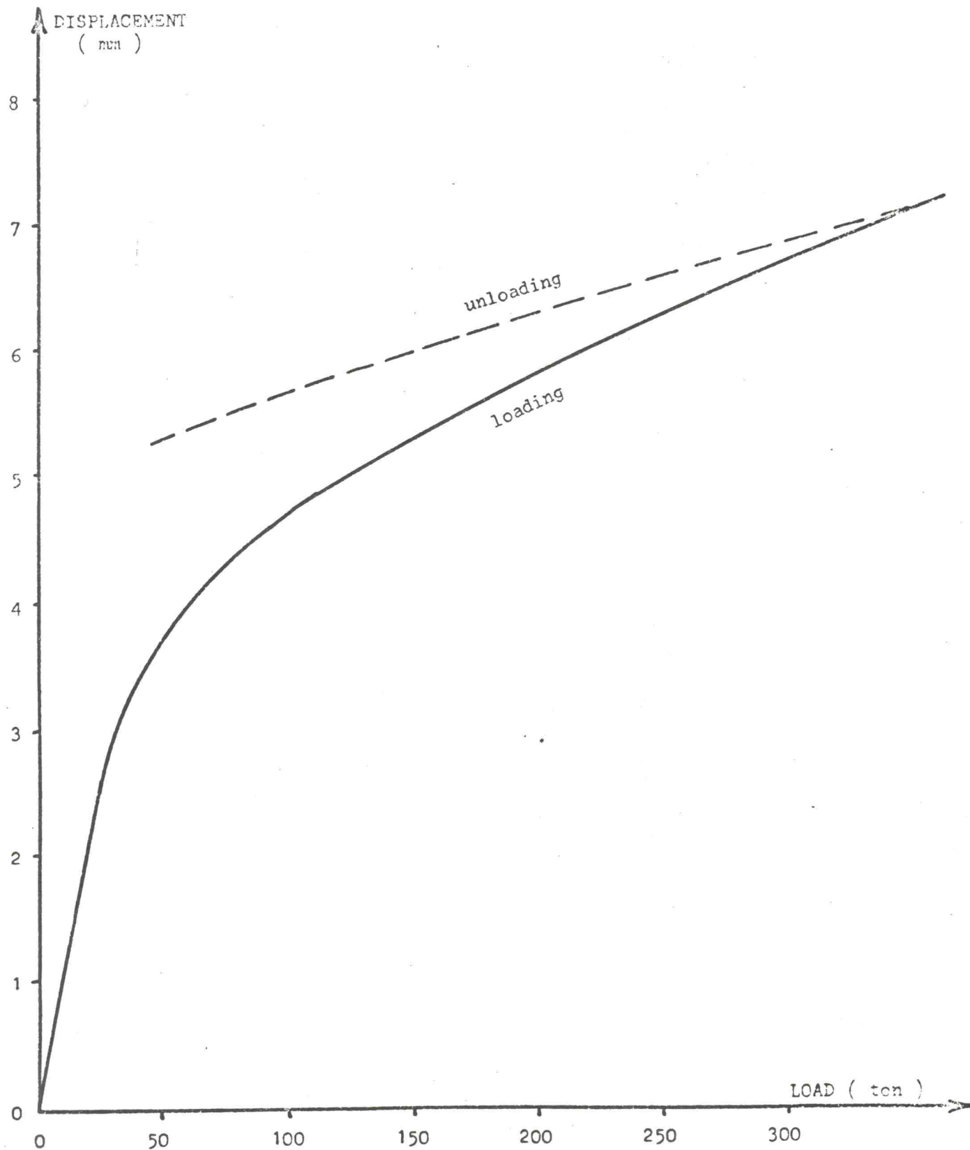
Figure 5. Piston displacement curve
