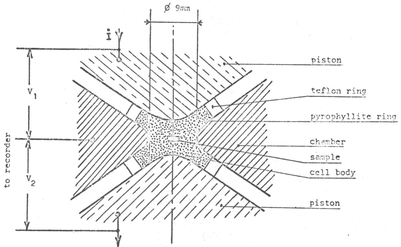
Figure 1 . Cross section of the cell inside the X type anvil
