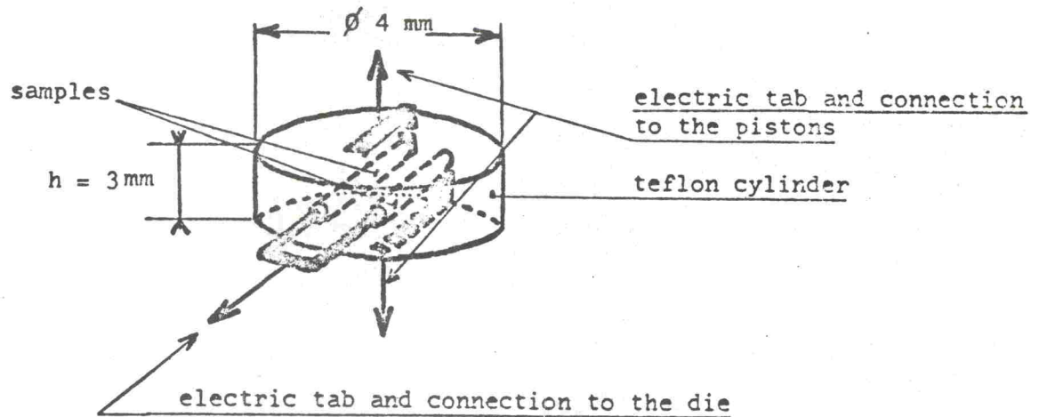
Figure 2 . Samples assembling, schematic
