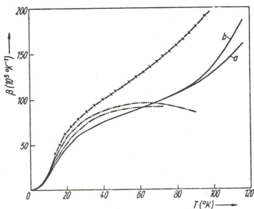
Fig. 3. Comparison of the experimental volume thermal expansion coefficient for Kr with theory (1). MLJ (12, 6) means (12, 6)-Mie-Lennard-Jones potential; qh: quasi-harmonic, anh: anharmonic approximation; a: measured with X-rays (9); b: bulk expansivity measured in this work
