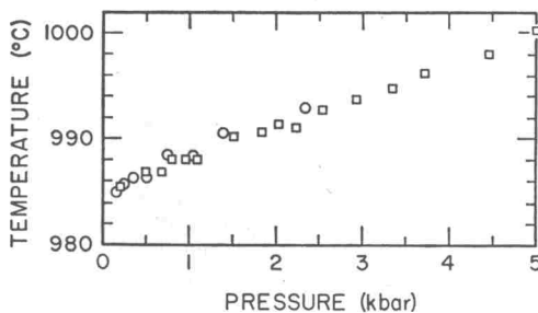
FIG. 1.—Temperatures for the transition in calcite at various pressures: circles denote data from the first run, squares those from the second run.
