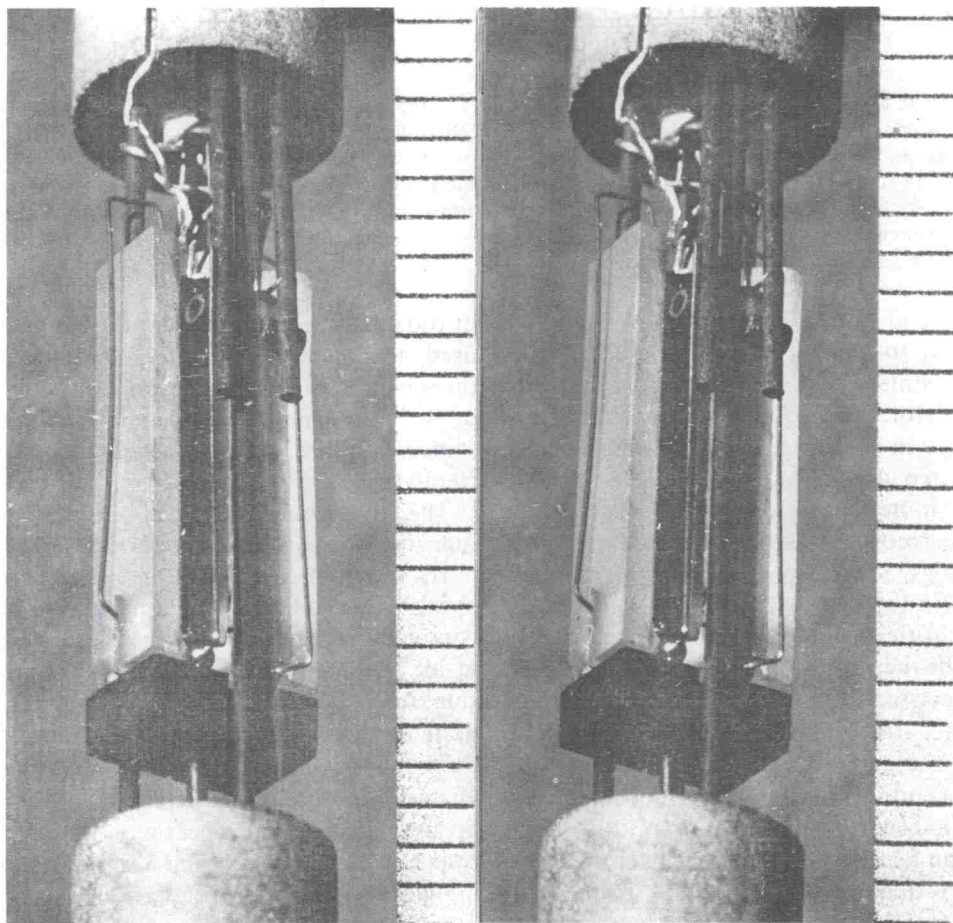
FIG. 5. Stereoscopic photograph of "gate"-type comparison dilatometer. Units on scale are millimeters. See Figure 6 for identification of parts.
