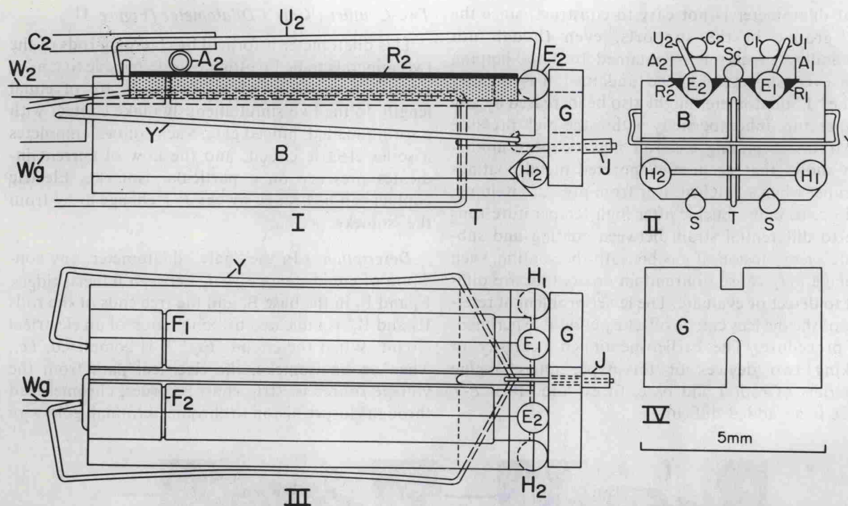
FIG. 6. Scale drawing of "gate" dilatometer. I. Side view, supports (S) removed for clarity. II. View from gate end with gate removed. III. View from top; some components removed for clarity. IV. Gate. Letters designate the following components: A 1 , A 2 —roller bearings; B—base; C 1 , C 2 —tungsten wires that clamp rods to fiducial ridge in base; E 1 , E 2 —electrical contact ball bearings; F 1 , F 2 —fiducial ridges; G—gate; H 1 , H 2 —hinge ball bearings; J—connection between gate and gate spring; R 1 , R 2 —rods of minerals being investigated; S—supports for dilatometer; T—thermocouple; U 1 , U 2 —spring clamps that keep electrical contact balls, E, in contact with rods, R, and also serve as part of the electric switch circuit; W 2 —electrical lead from closure piece to electrical contact ball, E 2 (note: W 1 not shown); W g —electrical lead, when connected, from gate to ground; Y—gate spring.
