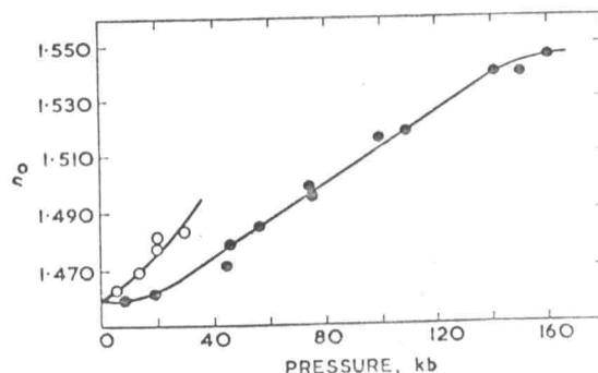
Fig. 1. Refractive index of silica glass measured at atmospheric pressure and room temperature as function of the pressure of the run ○ 600° ● 25°
