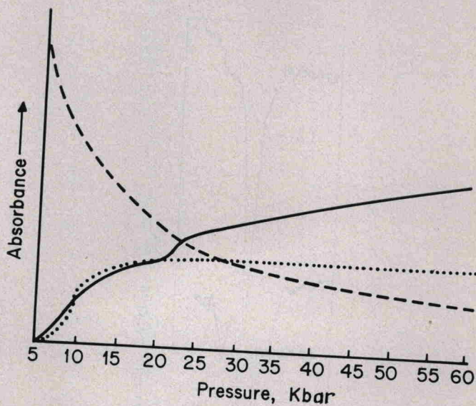
Fig. 2. Relative Intensity Changes in the \nu_4 Fundamental as a Function of Pressure [---, 715\text{ cm}^{-1} ; ..., 690\text{ cm}^{-1} ; —, 740\text{ cm}^{-1} ].
