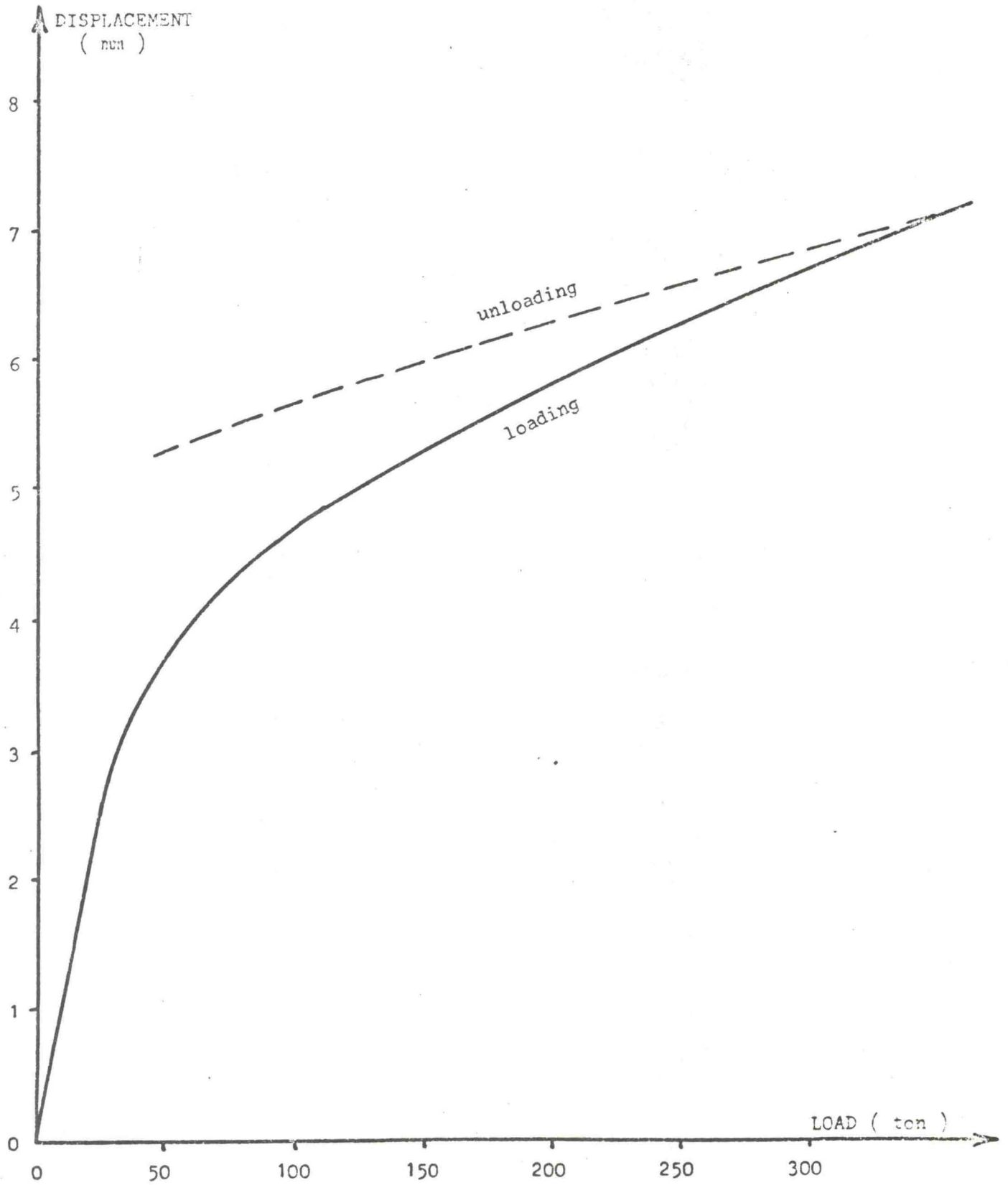
Figure 5. Piston displacement curve
