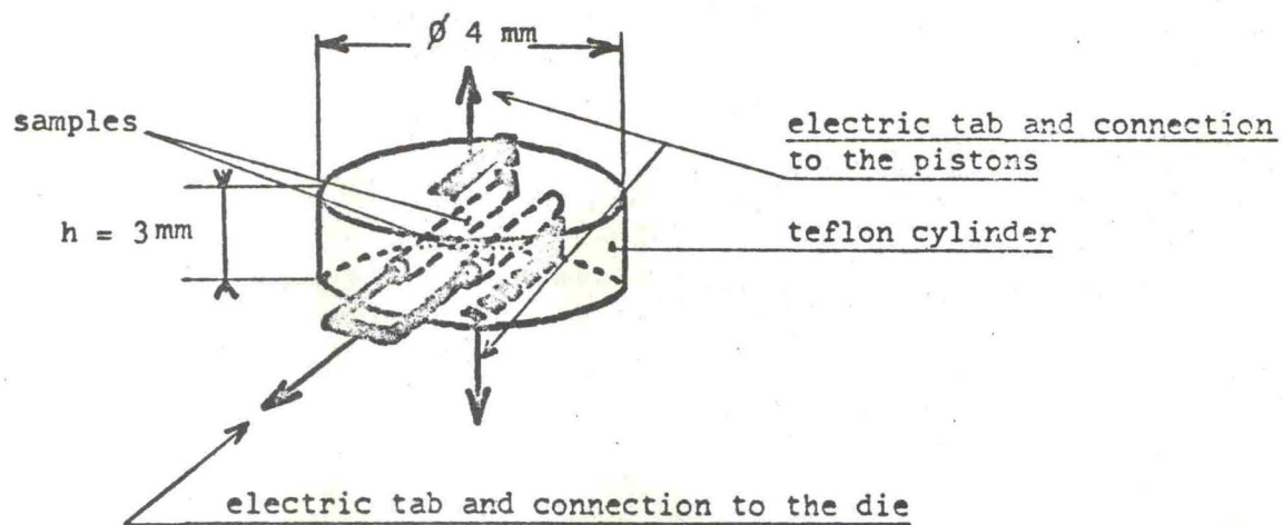
Figure 2 . Samples assembling, schematic
