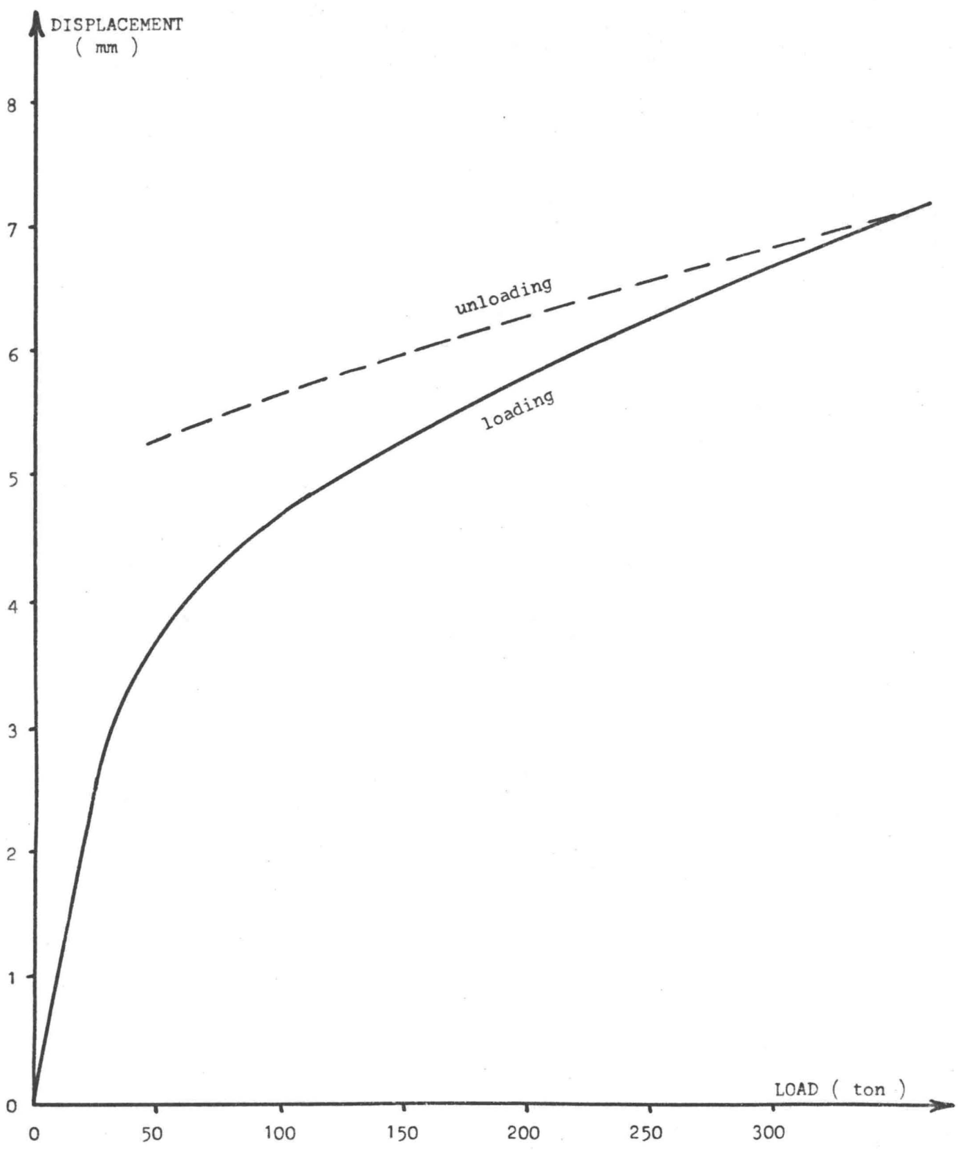
Figure 5. Piston displacement curve
