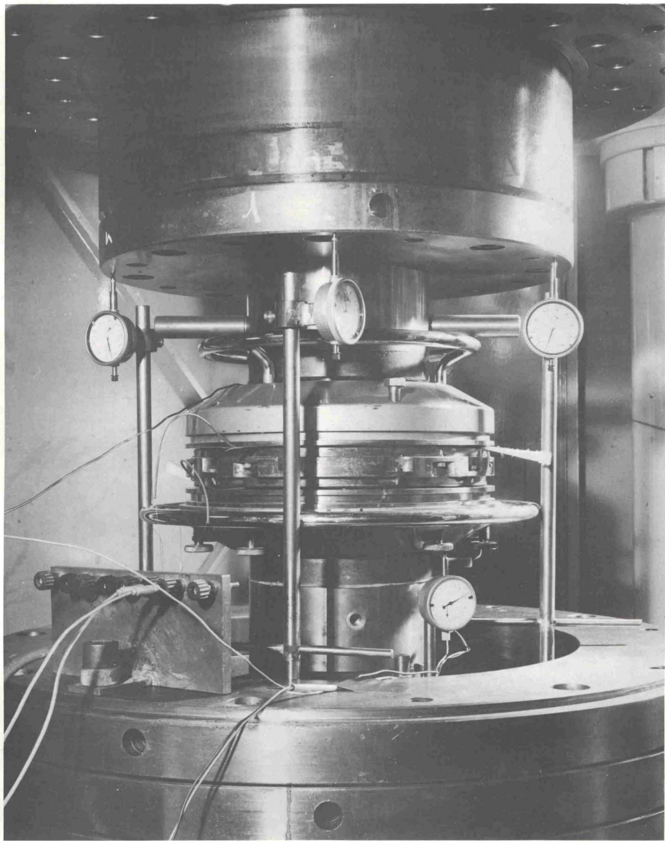
Figure 3 . Photograph of the "X type anvil" showing the four dial gages used to record the piston displacements
