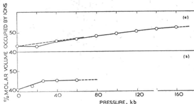
Fig. 6. Ratio of volume of the ions (Goldschmidt's radii) to the molar volume of the glass composition, measured at atmospheric pressure and room temperature, as function of the pressure of the run (a) SiO_2 25° (b) K_2O, 0.1MgO, 2.9SiO_2 500°
